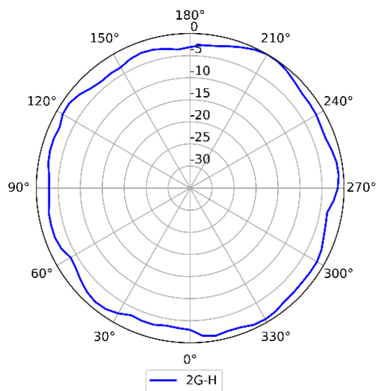
2.4GHz (Horizontal)
